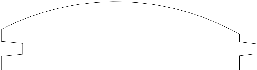
SIDING 95131 1 3/8" X 5 1/8" LAYS 4 3/4"
