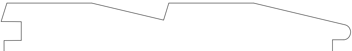
SIDING 95381 3/4" X 5 3/8" LAYS 5 1/16"
