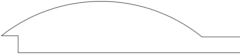
SIDING 935021 3/4" X 3 1/2" LAYS 3 1/4"
