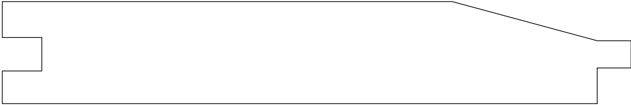
SIDING 955017 7/8" X 5 1/2" LAYS 5 1/4"
