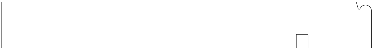
FACE FRAME 96001 3/4" X 6"
