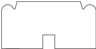
FACE FRAME 91503 3/4" X 1 1/2"
